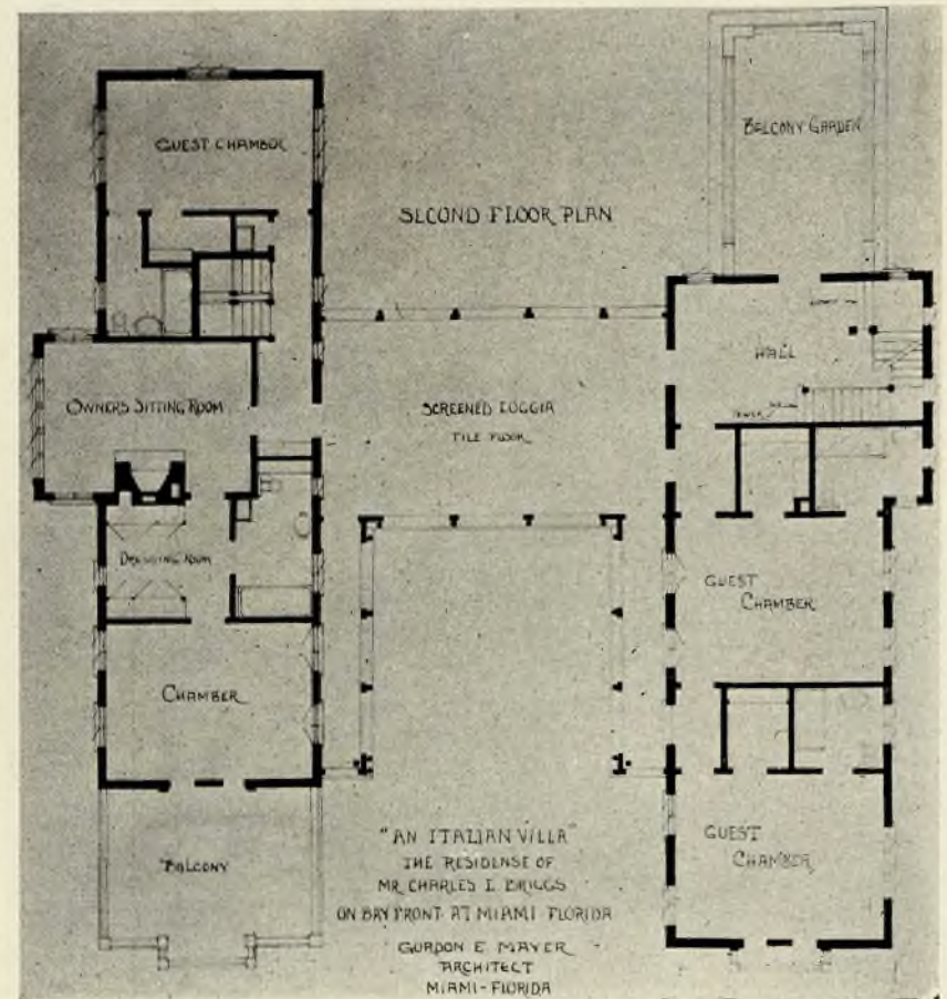
HOUSE OF CHARLES L. BRIGGS, MIAMI, FLORIDA GORDON E. MAYER, ARCHITECT
